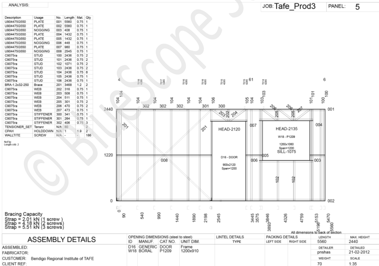
Figure 6.2 A typical wall frame assembly sheet as produced by ENDUROCADD®. The sections are branded when produced in accordance with Section 6.1 of this manual.
