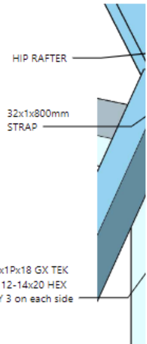
Figure 7.37. Tying down Veed hip ra
