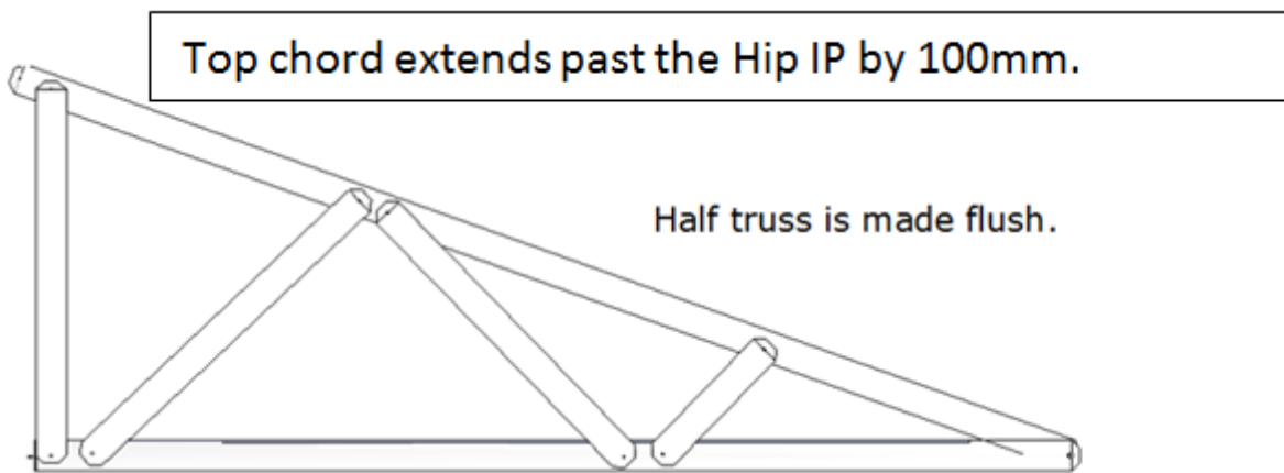
Figure 7.42: Hip truss
