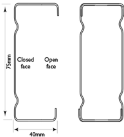
S75 section and boxed S75 section
