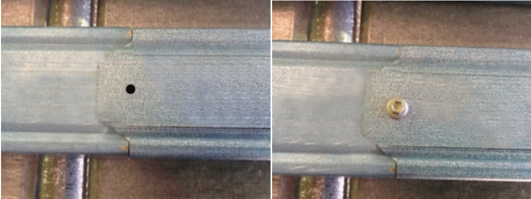
Figure 6.3 Bottom Chord connection at splice
