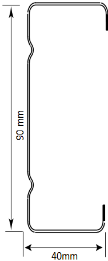
S90 Section
