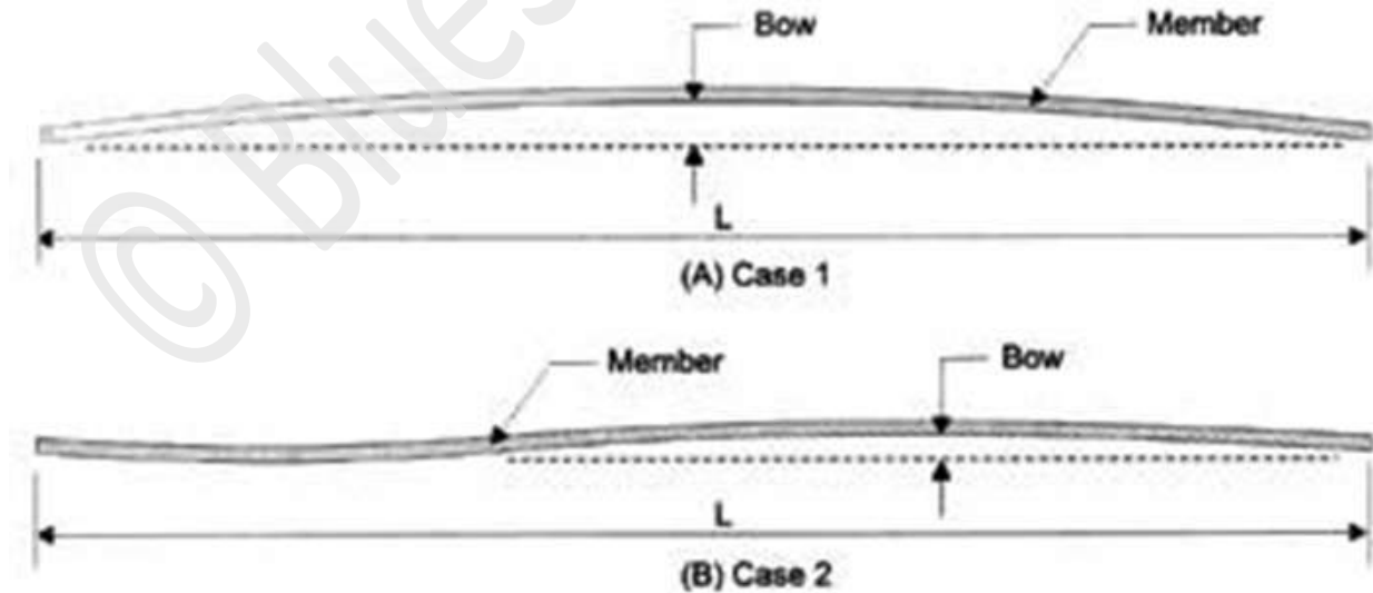
Detail: Straightness
