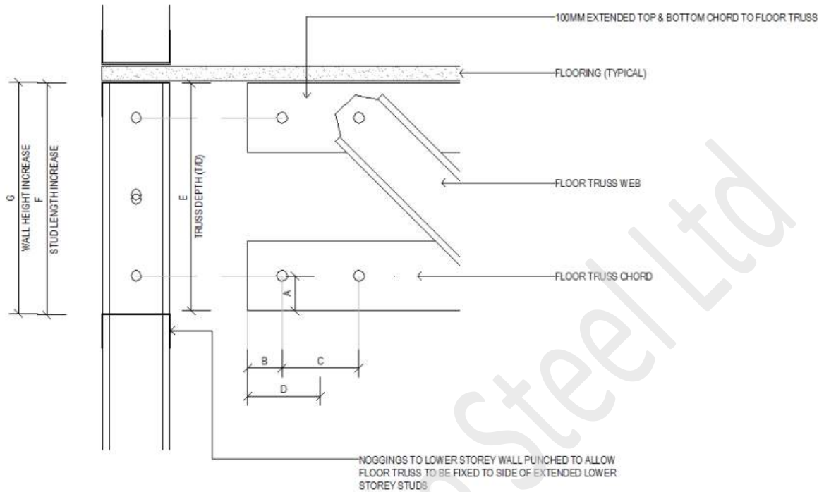
Detail: Floor truss component cribbing - Integrated wall system
