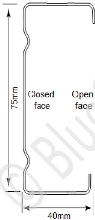
S75 Section
