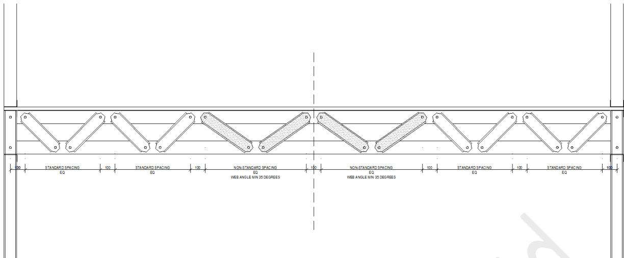
Detail: Typical standard floor truss - middle webs at minimum 35 degrees
