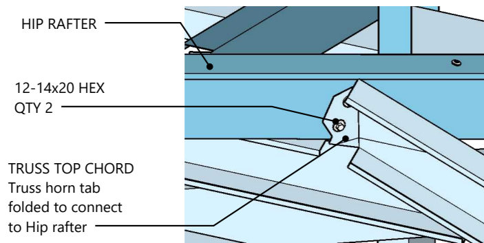
Truss horn to hip rafter connection
