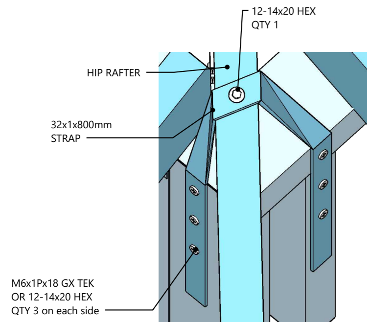
Hip rafter to wall tiedown
