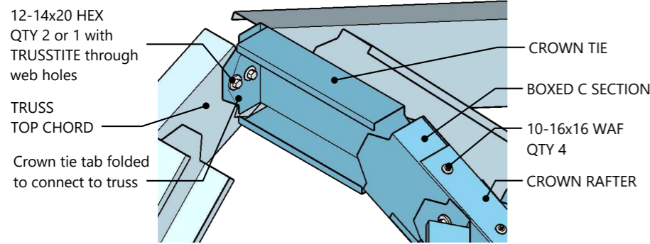
Crown rafter detail
