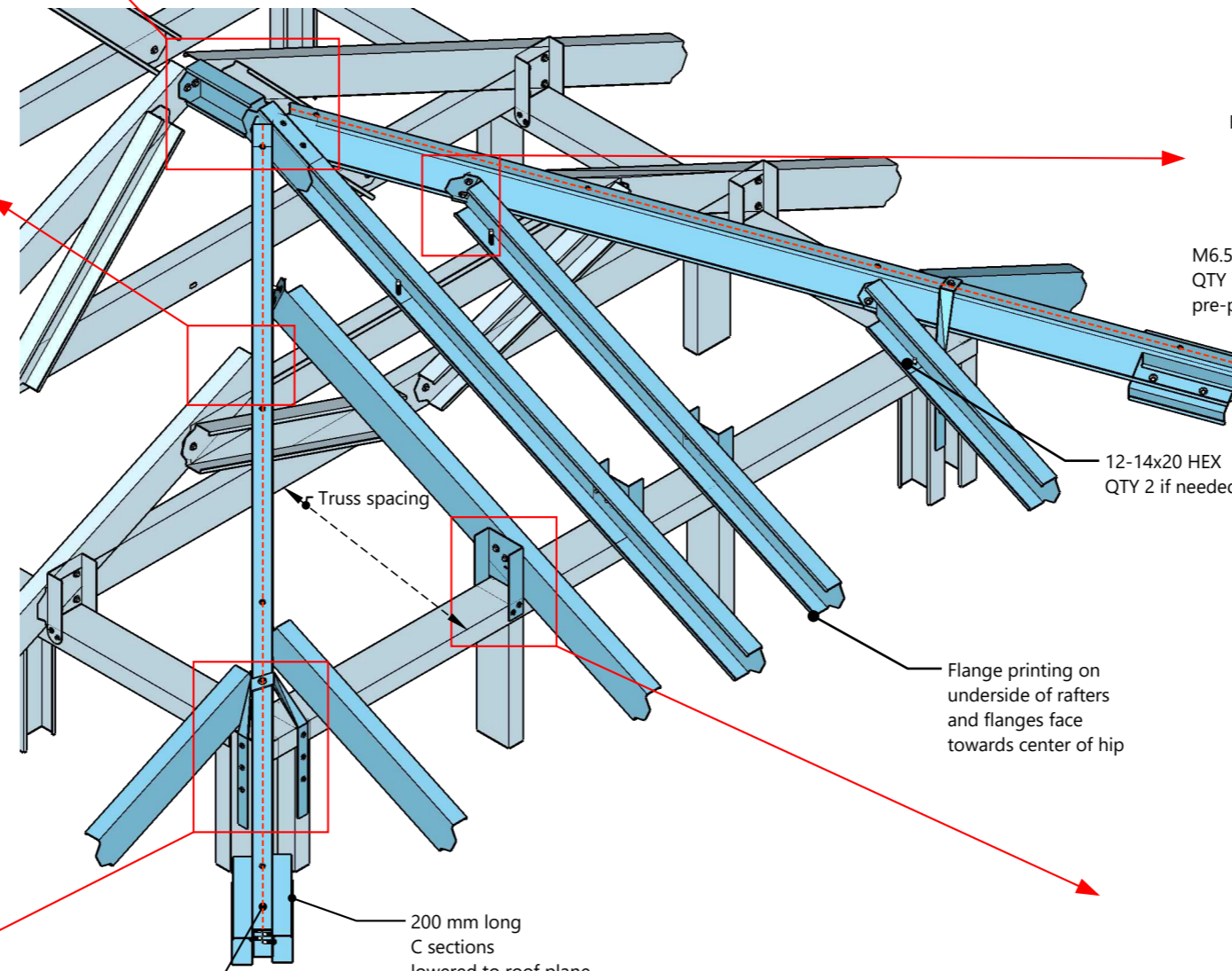
Truss horn to hip rafter connection
