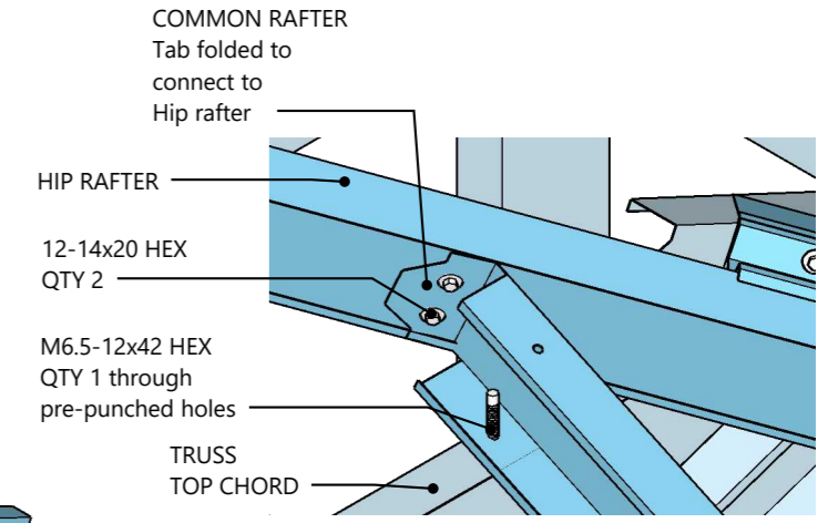
Common rafter detail
